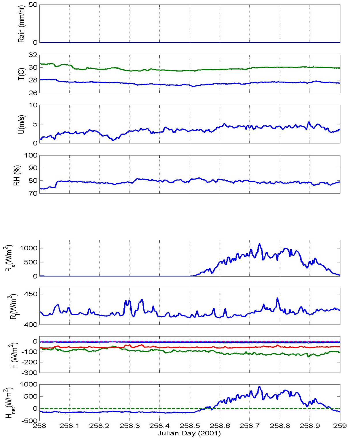
Figure D1. Bulk meteorology and flux variables from a typical clearish day in the tropics. Reading down from the upper panel the variables are: rain rate; water (green line) and air temperature (blue line); wind speed; relative humidity; downward solar flux; downward IR flux; heat flux components [ -H_s (blue), -H_l (green), R_{nl} (red), -H_{rain} (cyan)]; and net heat flux.
