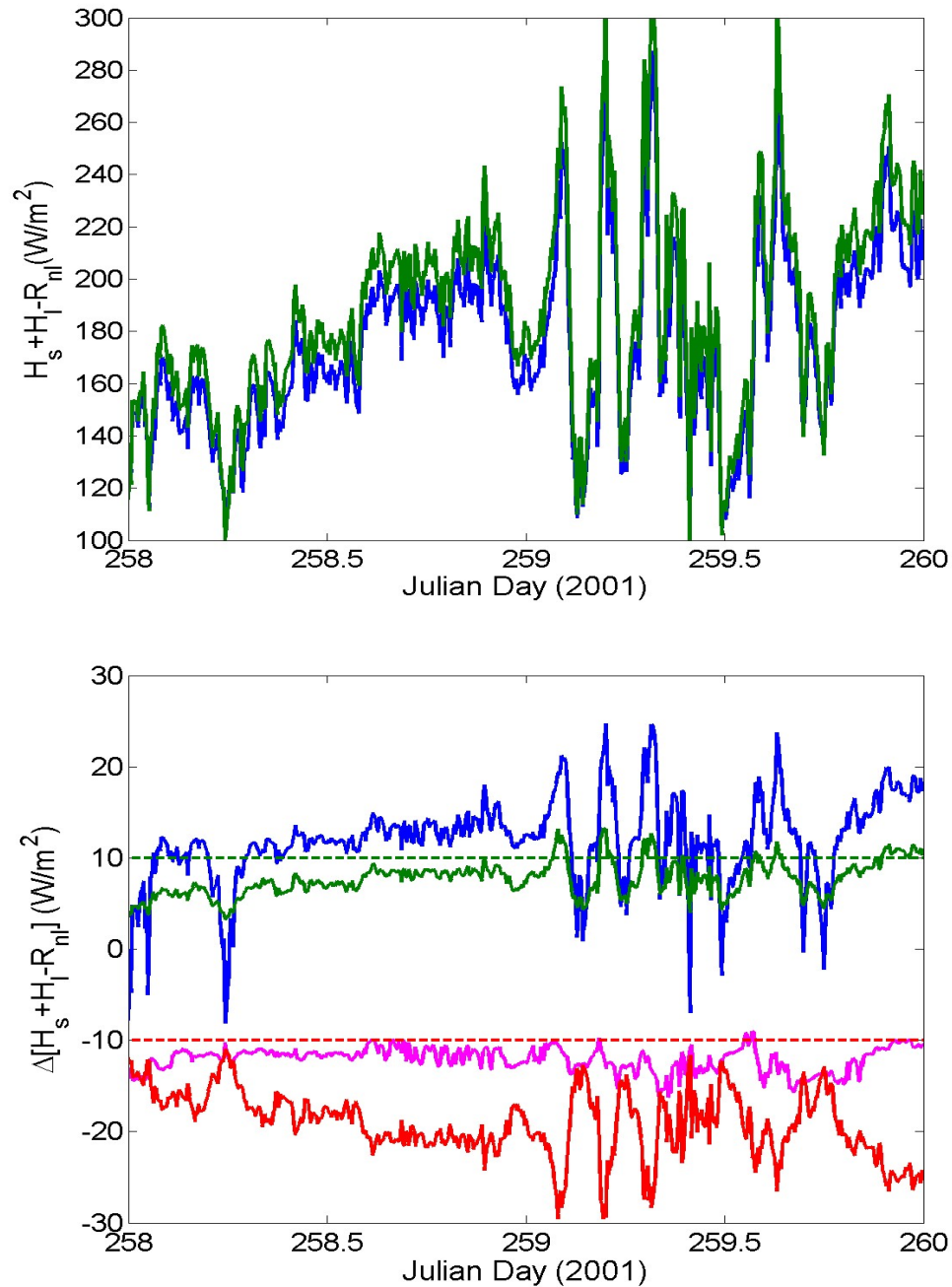
Figure 11.1. Sensitivity of bulk flux calculations to algorithm and input data; time series of sum of sensible, latent, and net longwave fluxes. Upper panel: COARE 3.0 (C3 blue) and Large and Pond (LP green). Lower panel: LP - C3 (blue), C3(Ts-0.5) - C3(Ts) (red), C3(qa-0.5) - C3(qa) (green), and C3(U - 0.5) - C3 (mauve).
