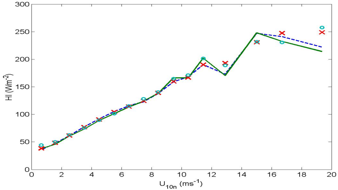
Fig. B2. The average of covariance and ID latent heat fluxes computed in 10-m neutral wind speed bins. Mean values are shown by lines and medians by symbols: the solid line and circles are measured fluxes, and the broken line and crosses are calculated with COARE 3.0.
