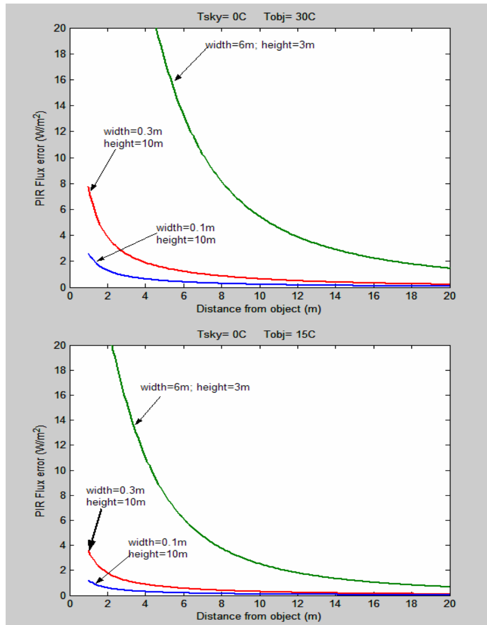
Figure C1. Longwave flux errors caused by shipboard objects in the field of view of a pyrgeometer; a tubular pole (blue), a mast (red), and a bulkhead (green). The assumed radiative sky temperature 0°C is typical of mid-latitude clear sky conditions. The lower panel is for an object at roughly ambient temperature; the upper panel is for an object warmed considerably by strong sun.
