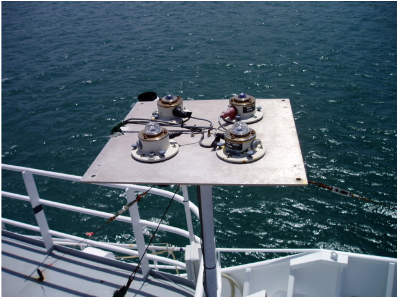
Figure 3.5 Example of duplicated pyranometer and pyrgeometer sensors mounted on a ship
