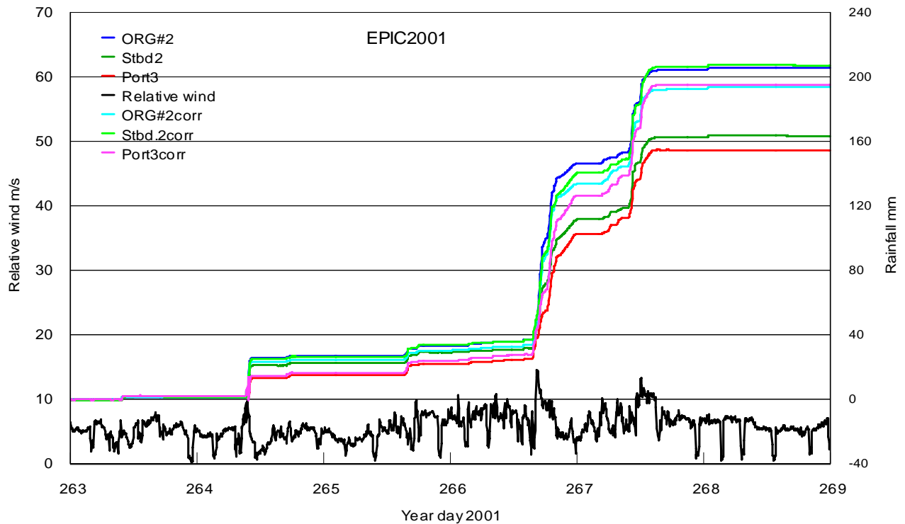
Figure 2.3. Cumulative rainfall measured by optical and funnel raingauges on a ship, before and after wind correction. The ORGs overestimate slightly when the raindrops are blown through the optical path at an angle to the vertical (dark and light blue traces). Siphon gauges underestimate when strong winds are distorted up over the ship and deflect raindrops away from the funnel (dark and light pairs of red and green traces). The black curve is the relative wind speed. Rainfall events started around day 264.4, 265.7, 266.6, and 267.3.
