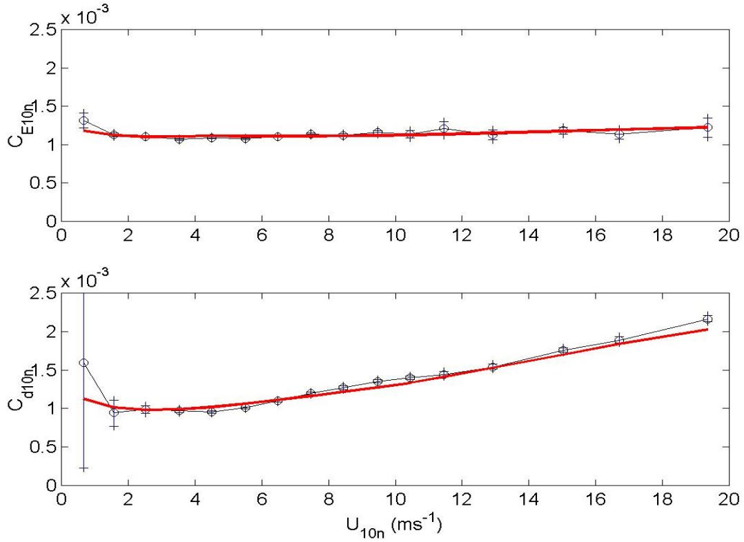
Fig. B1. Wind speed dependence of the momentum (lower panel) and scalar transfer (upper panel) coefficients for COARE versions 3.0 (solid line) and measurements (thin line with circles)
