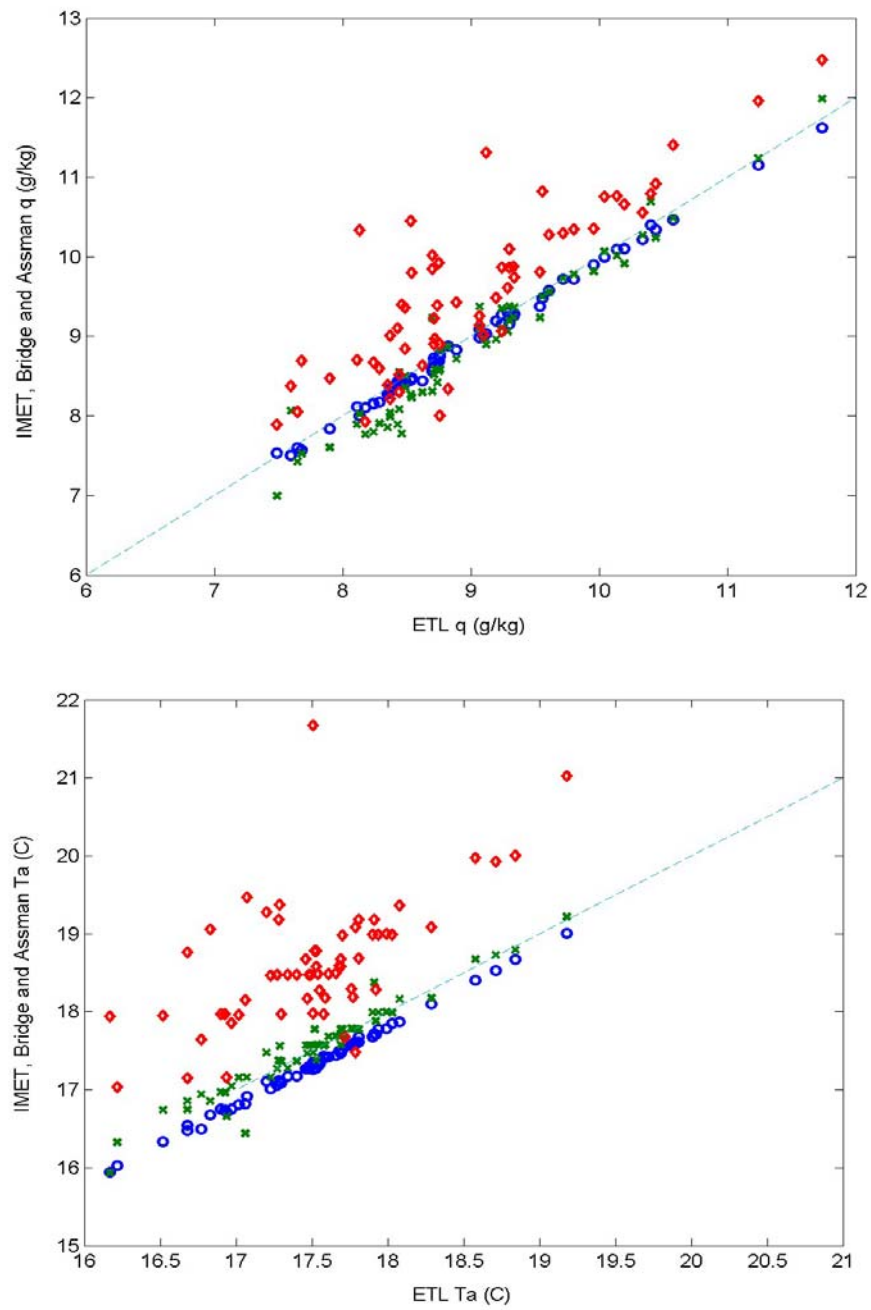
Figure 3.2. Comparison between a high quality T/RH sensor used by ETL and: (green symbols) an Assman psychrometer; (blue) the ship's IMET system; (red) the wet and dry bulb thermometers read by the bridge officers hourly for their weather reports.
