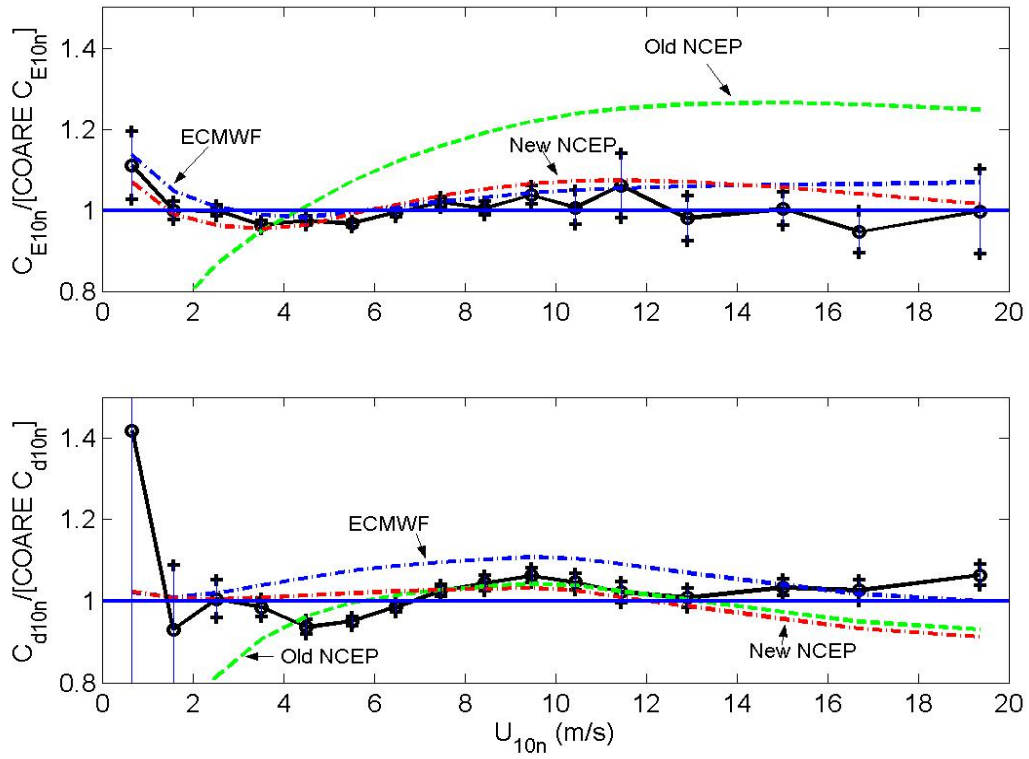
Fig. B3. The average wind speed dependence of 10-m neutral transfer coefficients divided by the COARE 3.0 values [Upper panel, C_{e10n} ; lower panel C_{d10n} ]. The dashed lines are NCEP and ECMWF formulae (as labeled); the solid line with symbols is the average ETL data.
