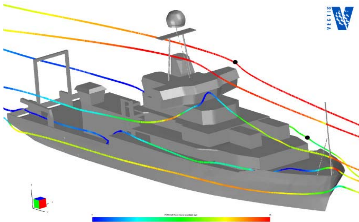
Figure 5.2 CFD simulation of wind flow around R/V Ron Brown . Positions of two funnel rain gauges are shown as black dots on particle trajectories which pass through them, showing the flow deflected sideways and upward at each site. Other trajectories originate 100m upwind on the centreline of the ship, at heights of 5, 7, 9, and 15 m above the sea surface. The colours represent wind speed and scale from 5 to 15 ms -1 . Courtesy Ben Moat.
