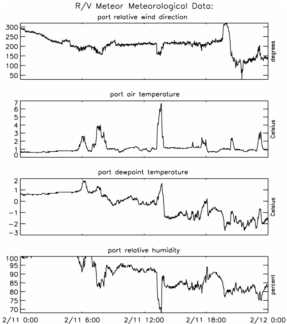
Figure 5.2. One-minute sampled relative wind direction, air and dewpoint temperature, and relative humidity from the scientific instrument system on the RV Meteor. Data are all from the port side sensors collected on 11 February 1990. The increases in air and dewpoint temperature and the decrease in relative humidity occur when the relative winds are from the stern ( \sim 160\text{--}200^\circ ) indicating contamination of the sensors by the vessel exhaust.
