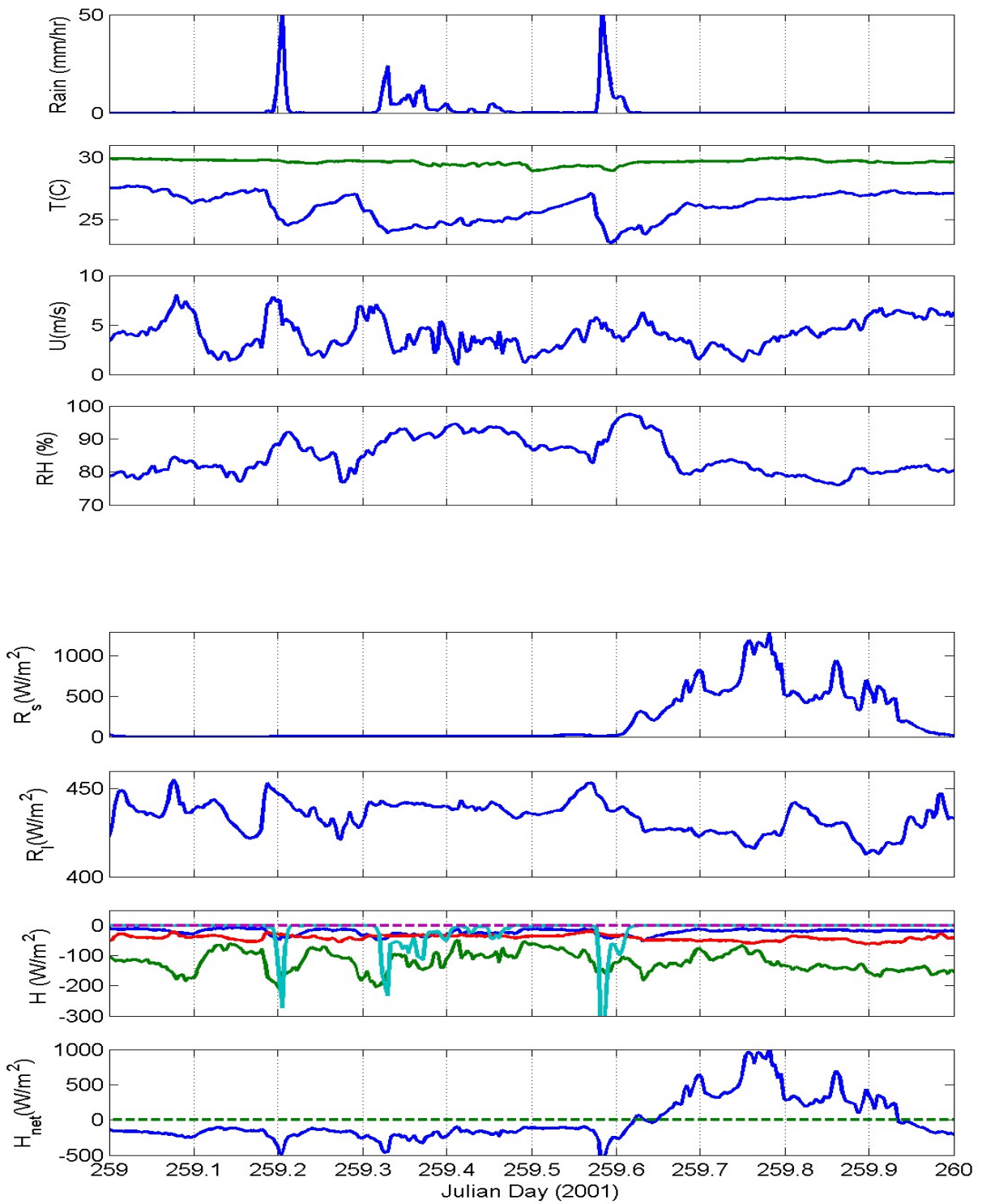
Figure D2. Bulk meteorology and flux variables for a convectively active day in the tropics. Reading down from the upper panel the variables are: rain rate; water (green line) and air temperature (blue line); wind speed; relative humidity; downward solar flux; downward IR flux; heat flux components [ -H_s (blue), -H_l (green), R_{nl} (red), -H_{rain} (cyan)]; and net heat flux.
