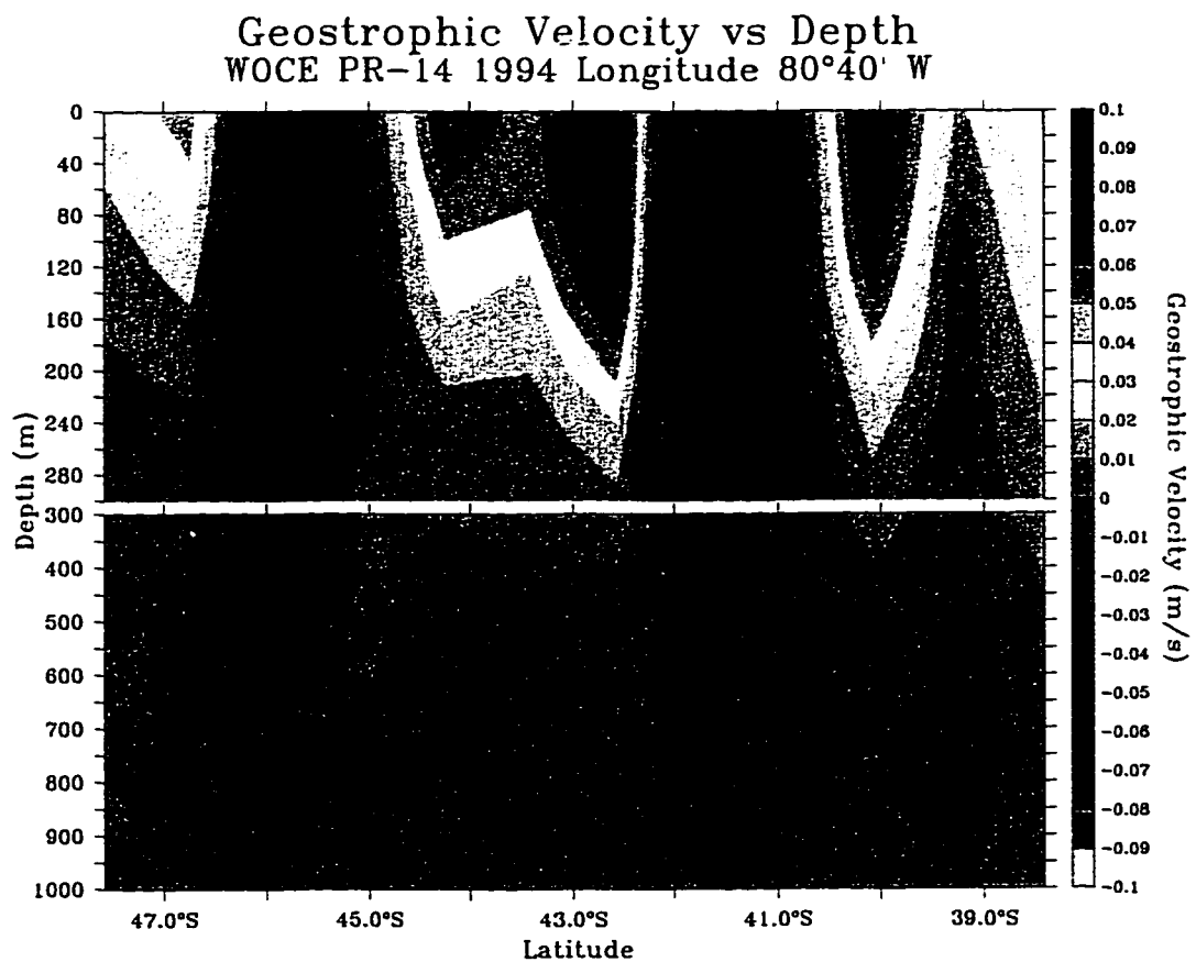
Figure 18: Vertical distribution of geostrophic velocity along longitude 080° 40' West during WOCE cruise PR-14 in 1994. Reference level (level of no motion) is 1000 meters. The upper part of the figure represents the first 300 meters of the water column. The bottom part goes from 300 to 1000 meters. Color bar on right-hand side indicates the geostrophic velocity in m/s. Positive values indicate eastward velocities.
