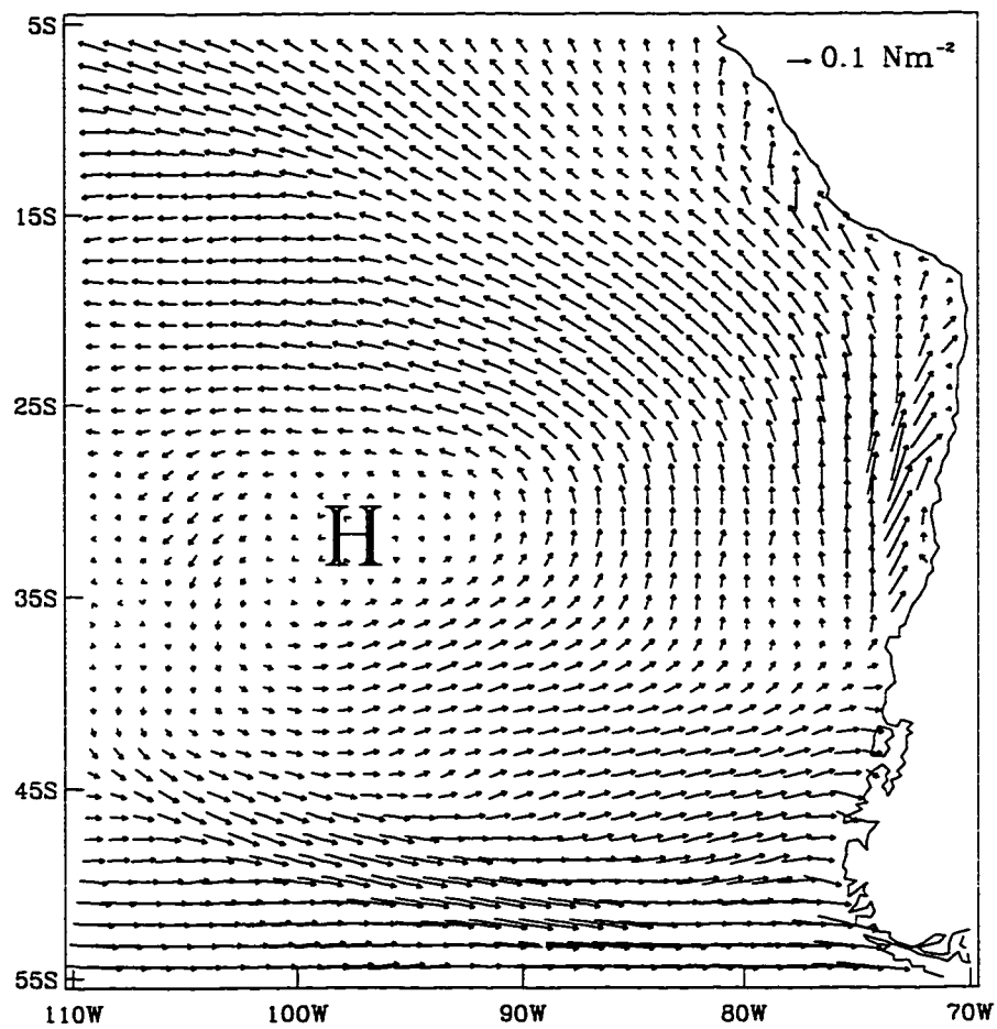
Figure 19: ECMWF averaged surface wind stress for the same period of the WOCE cruise PR-14 in 1994 (October 6 to October 22, 1994). The “H” indicates the location of the South Pacific High. A reference scale in \text{N/m}^2 is shown in the upper right corner.
