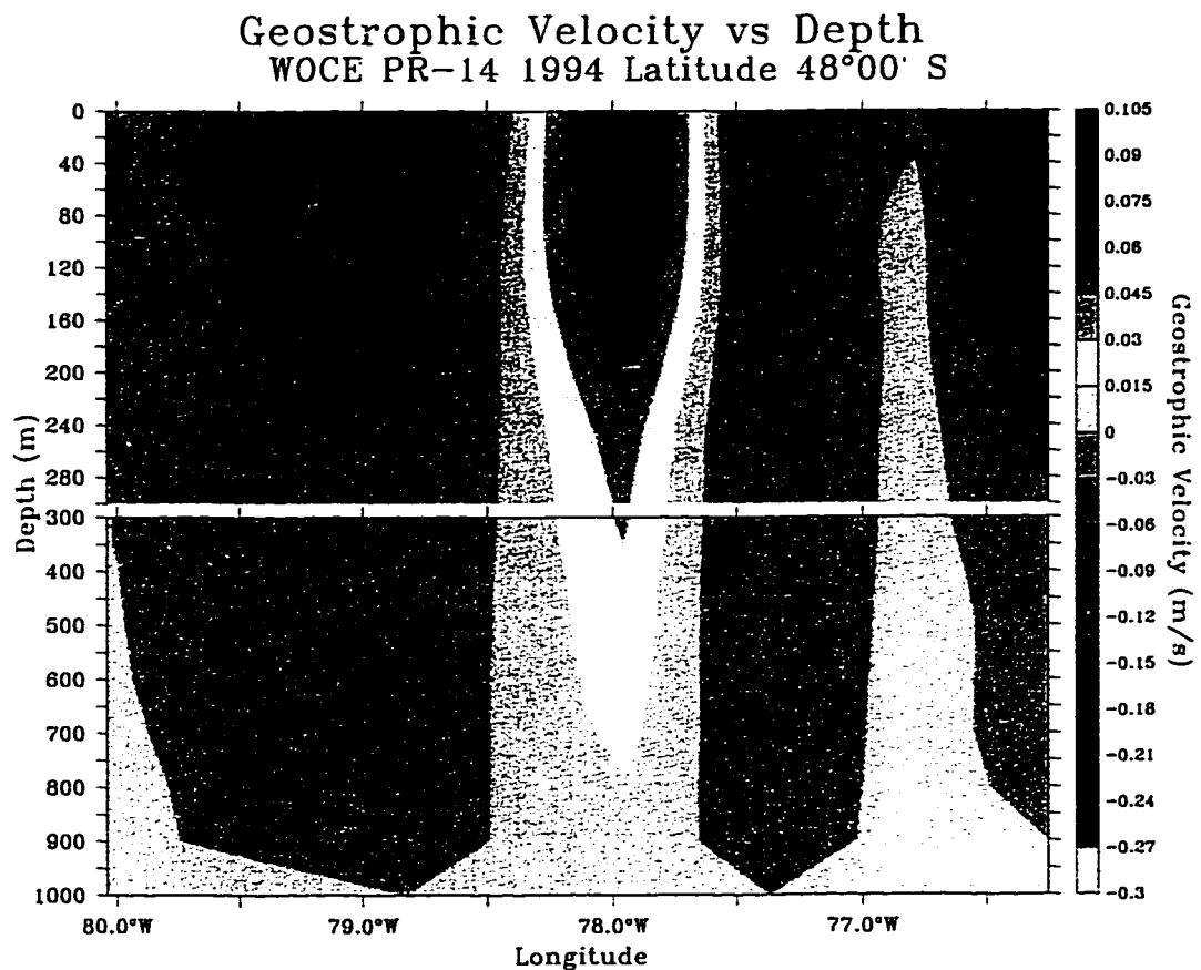
Figure 17: Cross-shelf section of geostrophic velocity at latitude 48° 00' South during WOCE cruise PR-14 in 1994. Reference level (level of no motion) is 1000 meters. The upper part of the figure represents the first 300 meters of the water column. The bottom part goes from 300 to 1000 meters. Color bar on right-hand side indicates the geostrophic velocity in m/s. Positive values indicate northward velocities.
