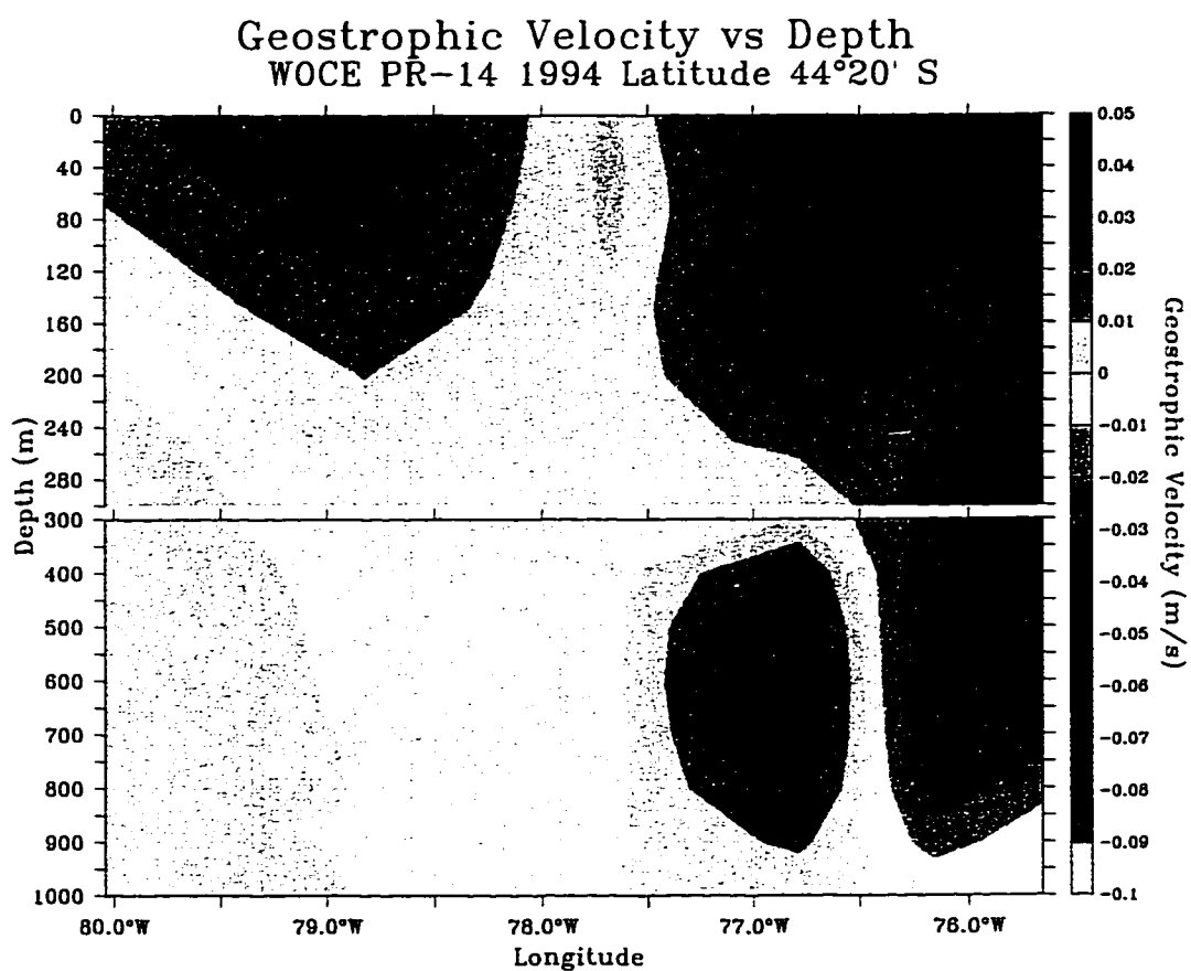
Figure 16: Cross-shelf section of geostrophic velocity at latitude 44° 20' South during WOCE cruise PR-14 in 1994. Reference level (level of no motion) is 1000 meters. The upper part of the figure represents the first 300 meters of the water column. The bottom part goes from 300 to 1000 meters. Color bar on right-hand side indicates the geostrophic velocity in m/s. Positive values indicate northward velocities.
