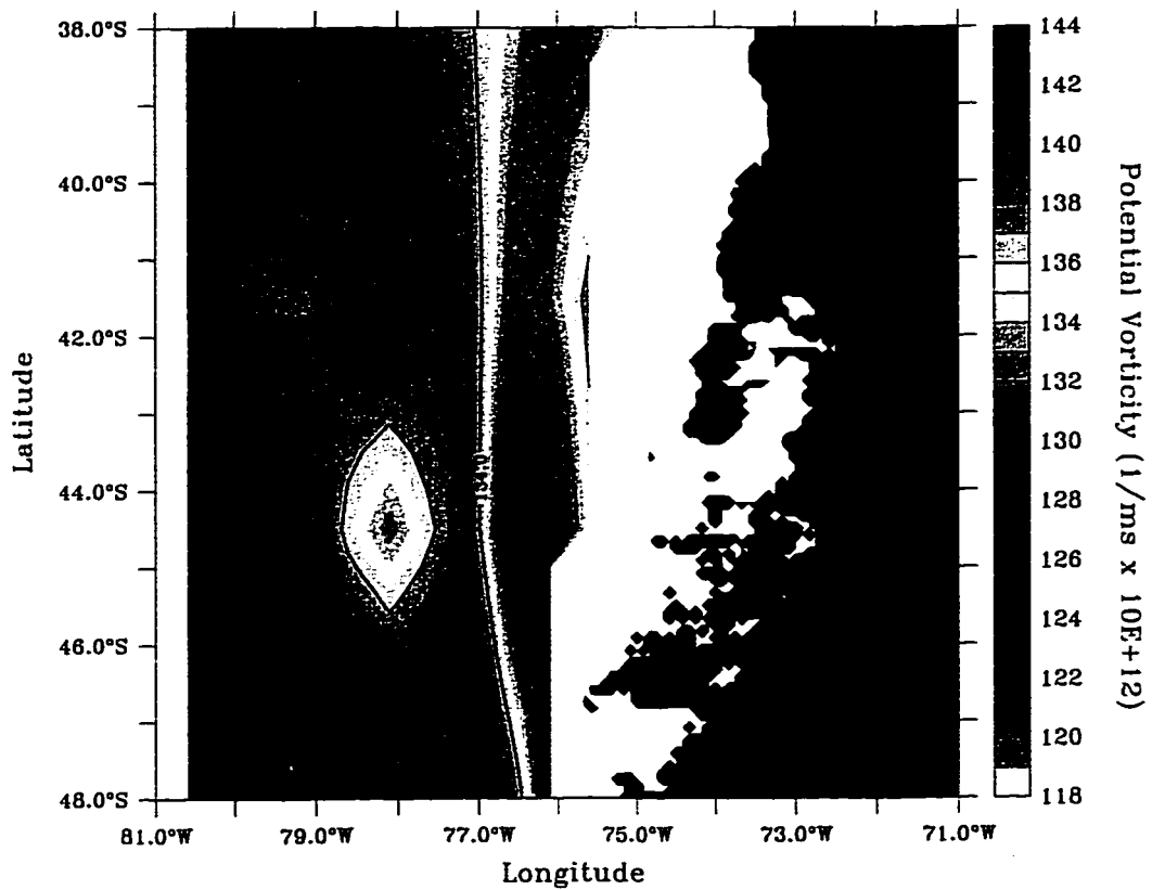
Figure 20: Interpolated potential vorticity field between \sigma_\theta = 26.2 \text{ kg/m}^3 and \sigma_\theta = 27.2 \text{ kg/m}^3 during WOCE cruise PR-14 in 1994. Contour lines are used to underline the proposed flow paths. Color bar on right-hand side indicates potential vorticity in 1/\text{ms} \times 10\text{E}+12 .
