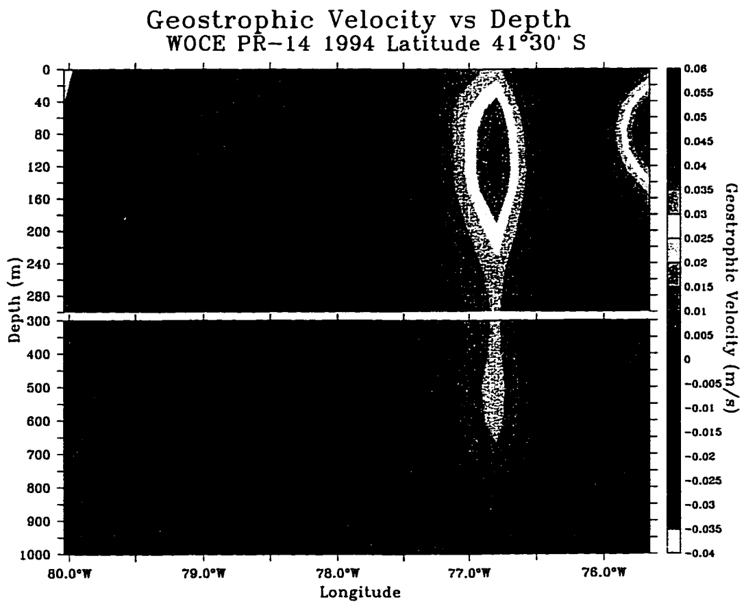
Figure 15: Cross-shelf section of geostrophic velocity at latitude 41° 30' South during WOCE cruise PR-14 in 1994. Reference level (level of no motion) is 1000 meters. The upper part of the figure represents the first 300 meters of the water column. The bottom part goes from 300 to 1000 meters. Color bar on right-hand side indicates the geostrophic velocity in m/s. Positive values indicate northward velocities.
