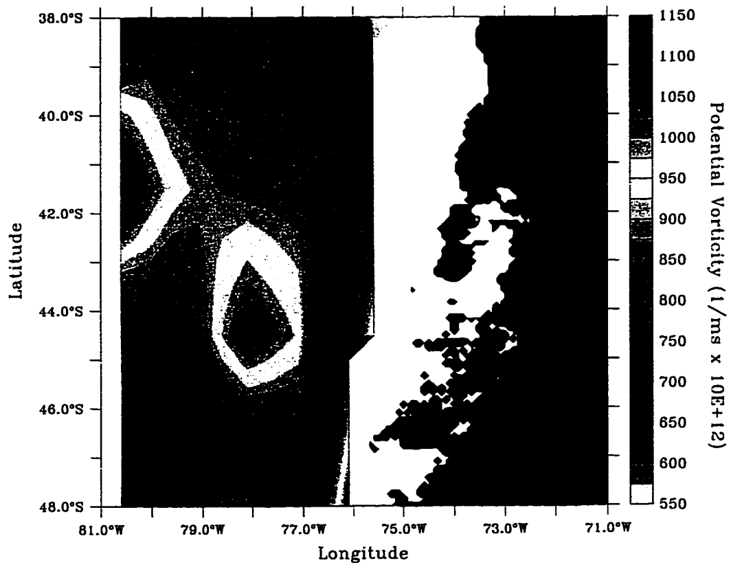
Figure 21: Interpolated potential vorticity field between \sigma_\theta = 26.2 \text{ kg/m}^3 and \sigma_\theta = 26.7 \text{ kg/m}^3 during WOCE cruise PR-14 in 1994. Contour lines are used to underline the proposed flow paths. Color bar on right-hand side indicates potential vorticity in 1/\text{ms} \times 10\text{E}+12 .
