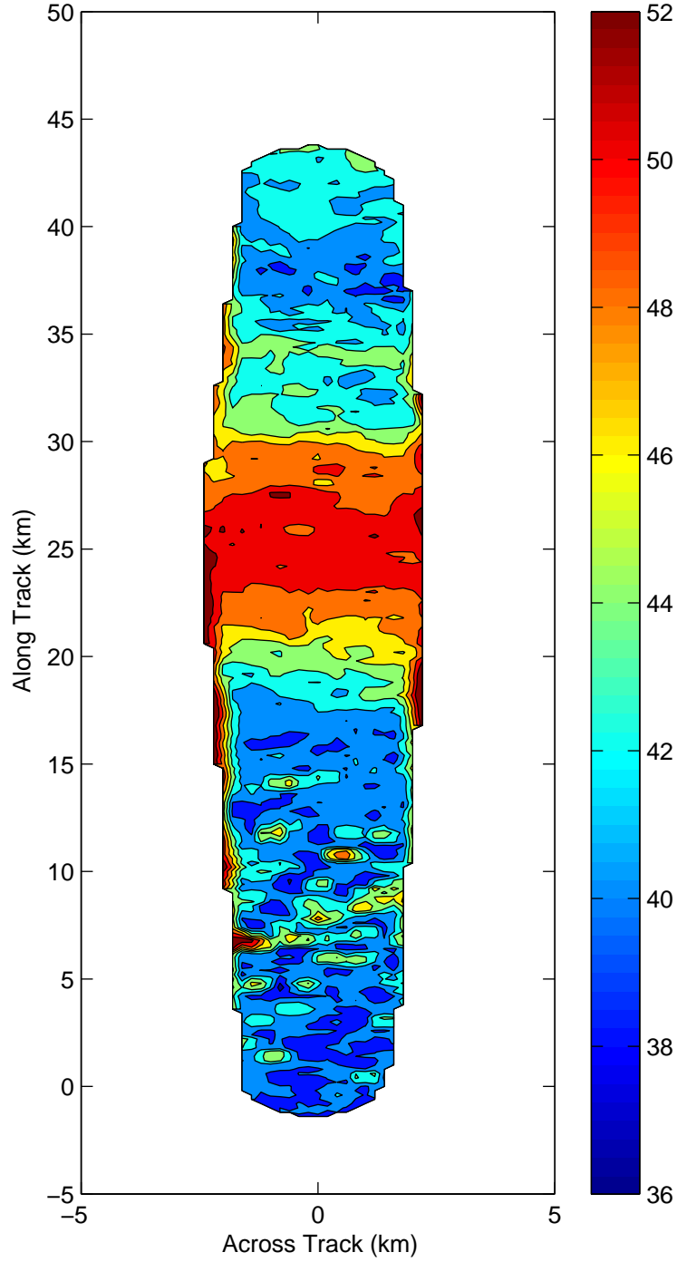
C band reflectivity at 630 meters height--Hurricane Isabel
