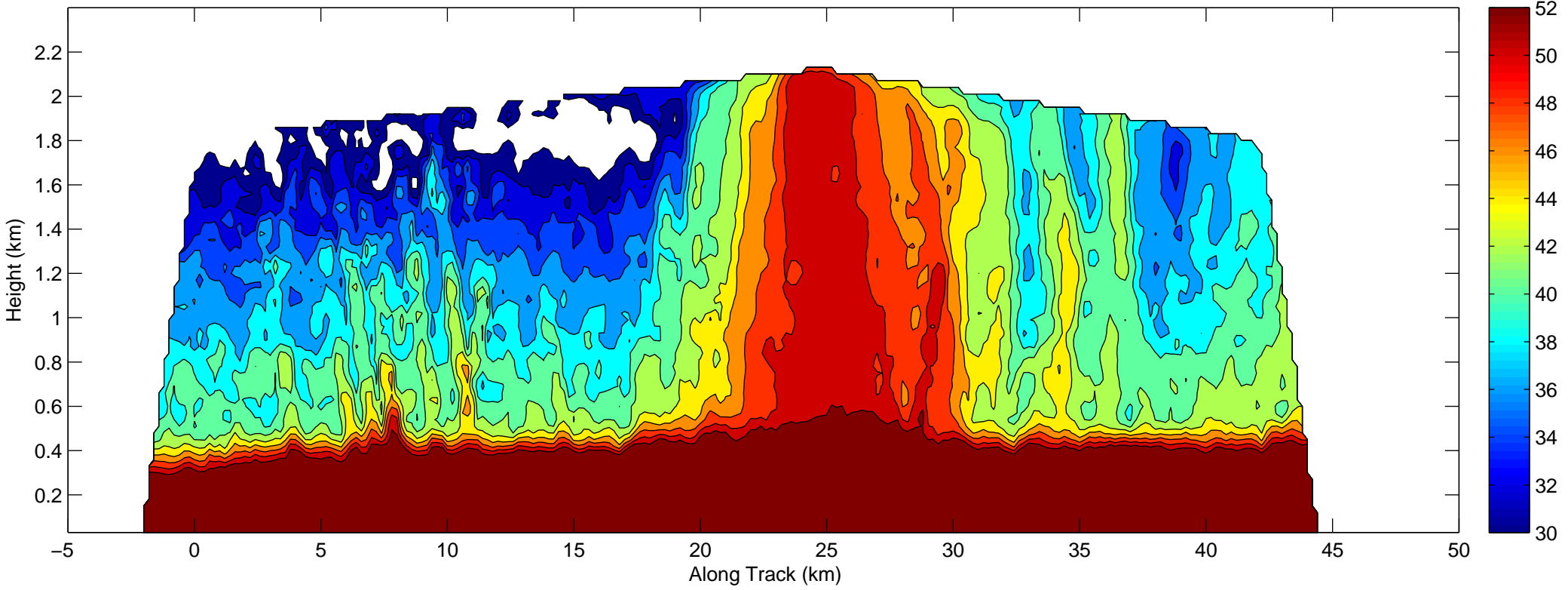
C band reflectivity cross section along aircraft track--Hurricane Isabel
