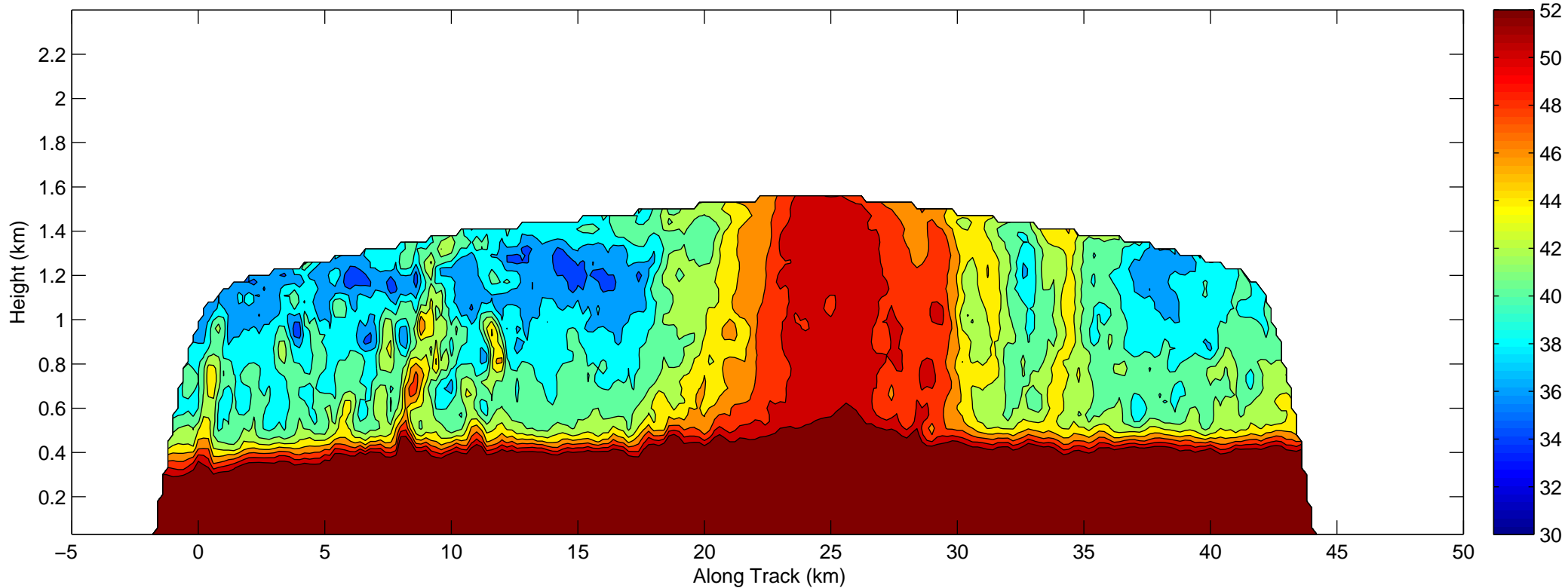
C band reflectivity cross section (1 km right of nadir)--Hurricane Isabel
