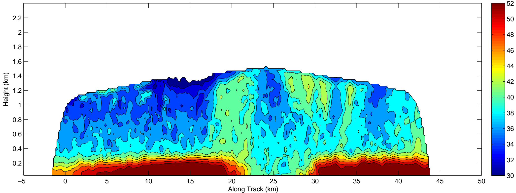
Ku band reflectivity cross section (1 km right of nadir)--Hurricane Isabel
