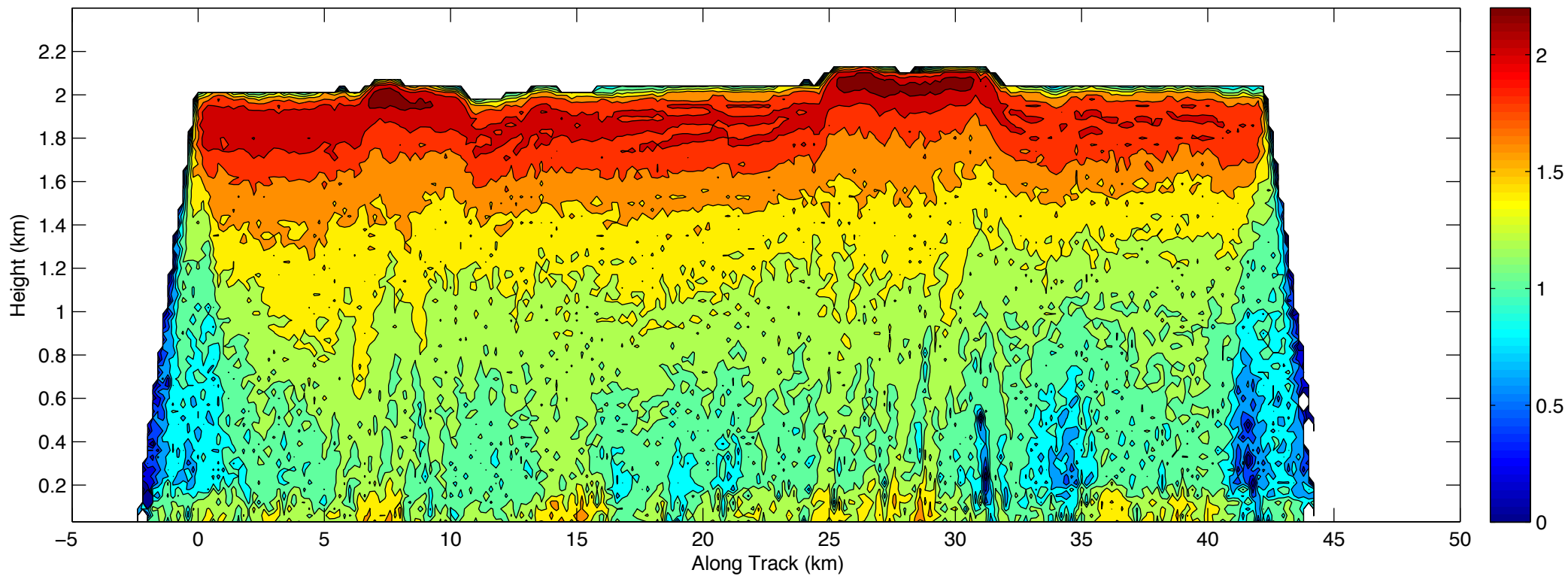
Number of pulses (log scale) in 200 m x 200 m x 30 m grid for all 4 beams at C Band Slice at nadir
