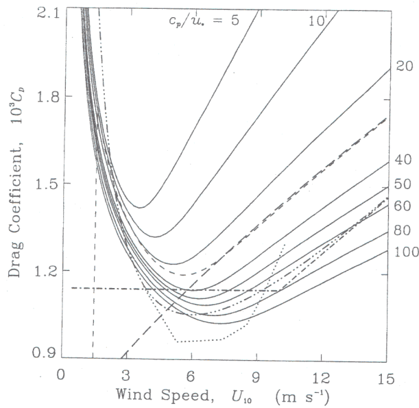
FIG. 8. Neutral drag coefficients for various wave ages ( c_p/u_* ), assuming the mean wind direction is parallel the mean direction of wave propagation. The values of wave age corresponding to the solid curves are given in the figure. The thin dashed curve is the modeled drag coefficients for wind-wave equilibrium ( c_p/u_* \approx 28 for U_{10} > 7 \text{ m s}^{-1} ); the vertical dashed line indicates the capillary cutoff. The thick dashed curve shows the Smith et al. (1992) drag coefficients. The dotted curve is the best fit to the SOFIA and SEMAPHORE data (from Dupuis et al. 1997; their Fig. 3a). Also shown are two empirical drag coefficients for the open ocean: the dot-dash (---) curve is Large and Pond (1981) and the dot-dot-dot-dash (----) curve is Large et al. (1995).
