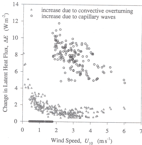
FIG. 9. Increased evaporation due to capillary waves (○) and convective overturning (Δ).
