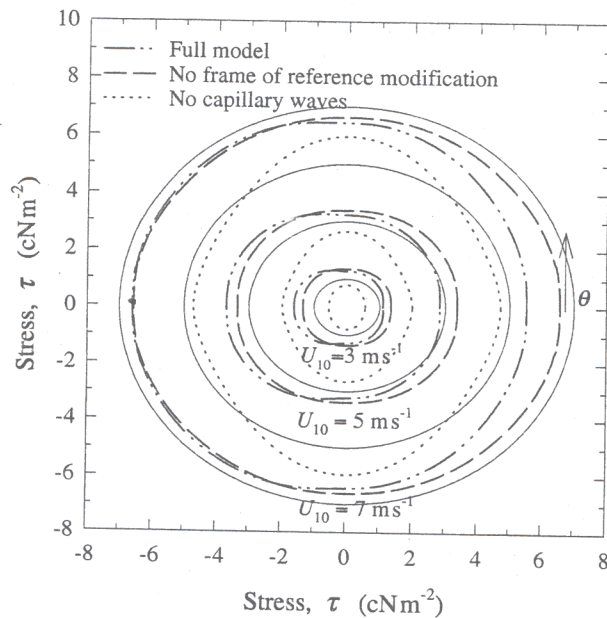
FIG. 4. Neutral stress magnitudes, as a function of the angle between the direction of the wind and the direction of wave propagation, for three wind speeds (3, 5, and 7 \text{m s}^{-1} ). The swell has a phase speed of 20 \text{m s}^{-1} . The dotted line indicates the stress ignoring capillary waves, the dashed line indicates the stress ignoring the frame of reference correction, and the dash-dot-dot line shows both considerations. The solid lines show stresses of 1, 3, 5, and 7 \text{cN m}^{-2} .
