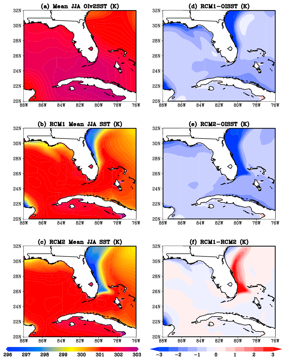
Figure 2. The climatological mean JJA SST (in K) from (a) observations (OISSTv2), (b) RCM1 integration, and (c) RCM2 integration. The corresponding systematic error (°C) of (d) RCM1 and (e) RCM2 and (f) the difference between RCM1 and RCM2.
