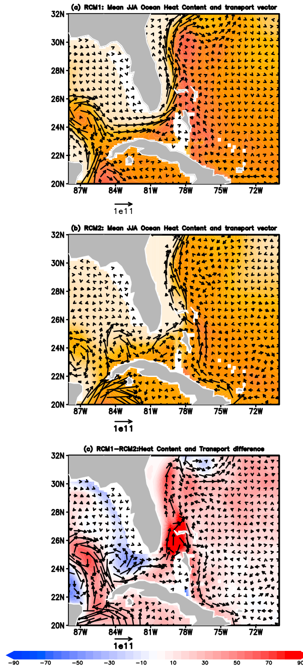
Figure 10. The climatological mean JJA ocean heat content as measured by the depth of the 20°C isotherm (in meters) overlaid with upper ocean heat transport vectors (equation 5 in text; \text{W m}^{-1} ) from (a) RCM1, (b) RCM2, and (c) RCM1 – RCM2 (Figure 10a minus Figure 10b).
